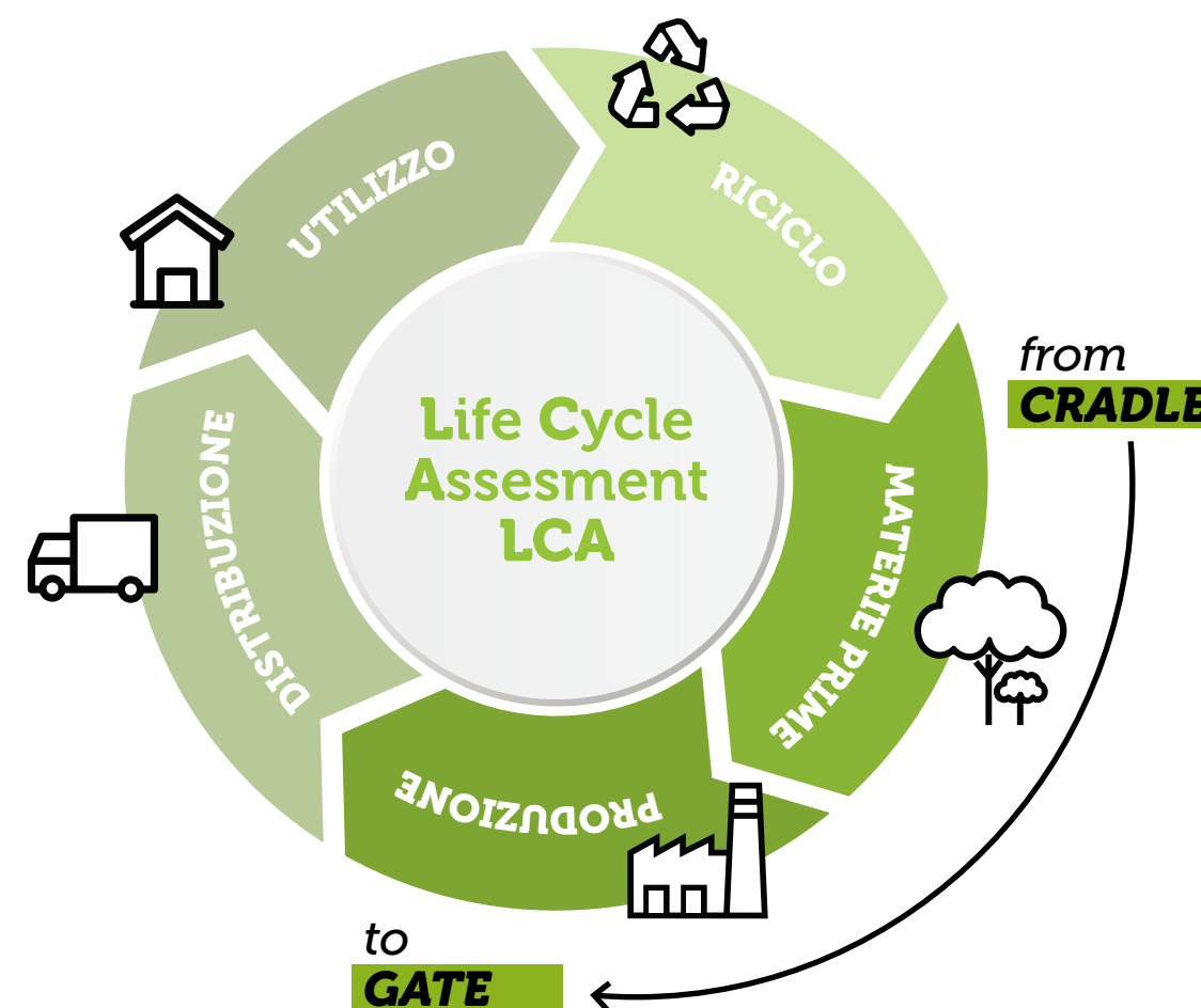
Figura 15: Life Cycle Assessment – cradle to gate
